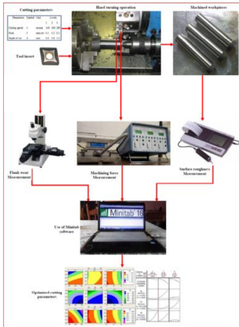
Fig1. Experimental setup
